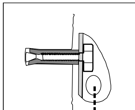
Figure 4: A self-drill that is underdrilled, but has a torqued bolt. Since a preload exists, it experiences only axial tension, bending, and shear.
